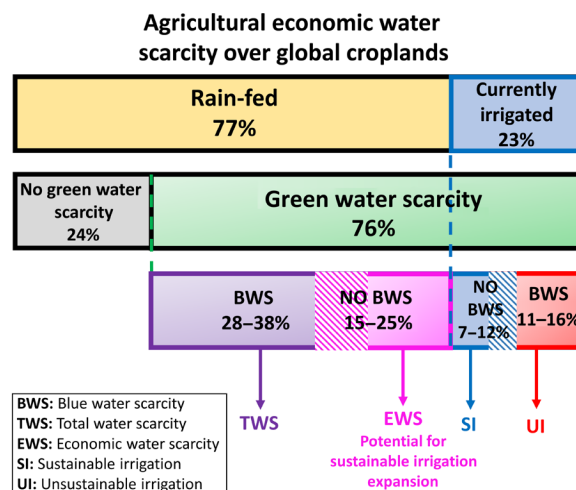
Fig. 1. Conceptual framework and extent of agricultural EWS. Percentages represent fraction of the global cultivated area in each category. Shading indicates croplands affected by blue water scarcity (BWS) that can be sustainably irrigated with deficit irrigation. These areas are then reclassified as suitable for sustainable irrigation [i.e., with no blue water scarcity (NO BWS)], considering different deficit irrigation scenarios. Lack of irrigation in these areas is interpreted as agricultural EWS. See Box 1 for concepts and definitions about agricultural EWS.
